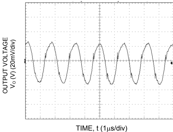
Fig-15. Typical output ripple and noise (C o =22μF ceramic, VIN = 12V, I o = I o,max ).
