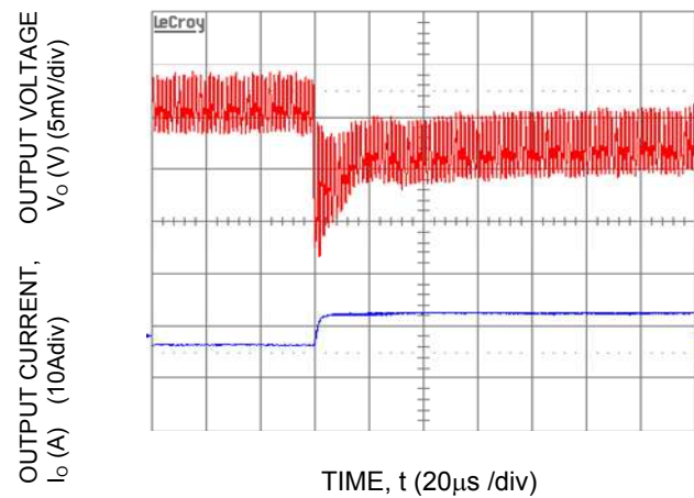
Fig-46. Transient Response to Dynamic Load Change from 50% to 100% at 12Vin, C out -3x47µF+6x330µF, CT tune -47nF, RT tune -180ohms
