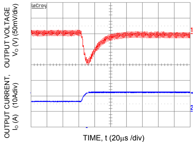
Fig-16. Transient Response to Dynamic Load Change from 50% to 100% at 12Vin, Cout-5x47uF, CTune-1500pF & RTune-330ohms
