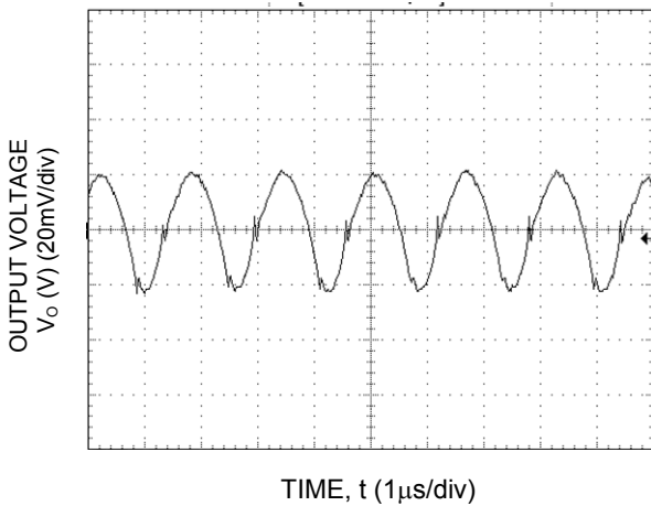
Fig-21. Typical output ripple and noise ( C_o=22\mu F ceramic, V_{IN} = 12V , I_o = I_{o,max} ).
