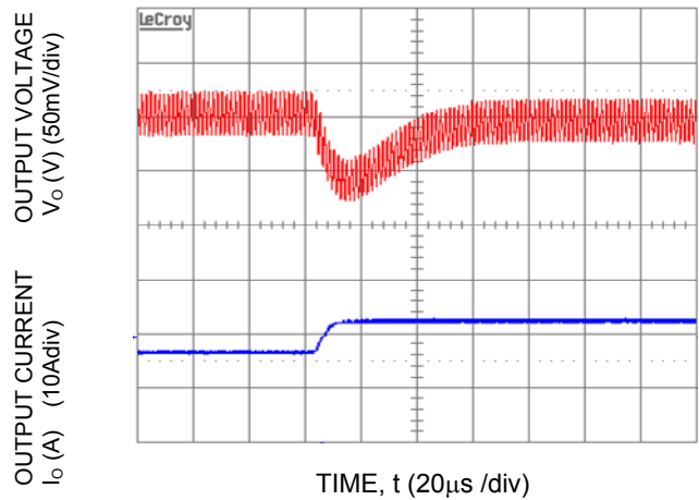
Fig-22. Transient Response to Dynamic Load Change from 50% to 100% at 12Vin, Cout-1x47 \mu F+1x330 \mu F, CTune-2700pF & RTune-330ohms
