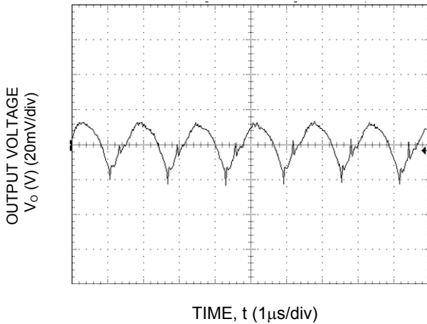
Fig-33. Typical output ripple and noise (C o =22µF ceramic, V IN = 12V, I o = I o,max .)
