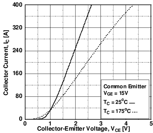
Figure 3. Typical Saturation Voltage
