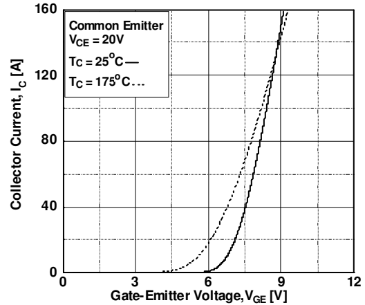
Figure 4. Transfer Characteristics
