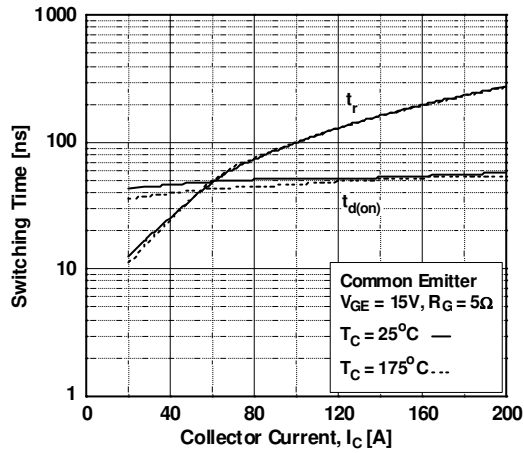
Figure 15. Turn-on Charateristics vs. Collector Current
