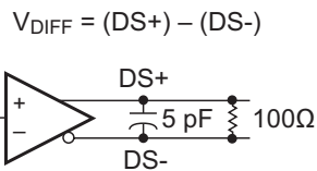
Figure 17. CTL Output Load and Transition Times
