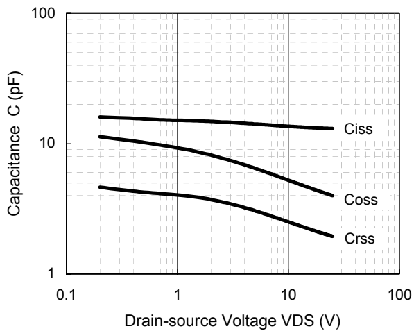
Capacitance - VDS
