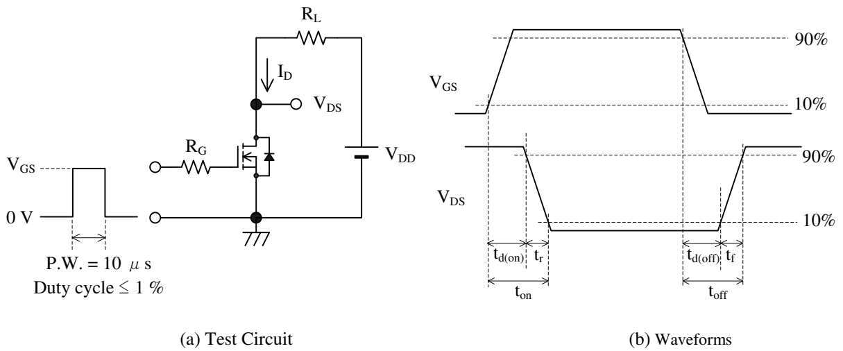
Figure 2 Switching Time
