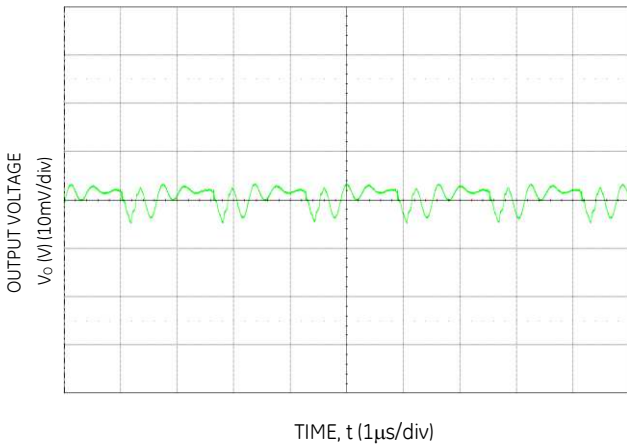
Figure 9. Typical output ripple and noise (C o =88μF ceramic, V IN = 12V, I o = I o,max ).
