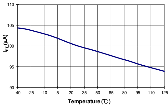
Figure 23. Internal Source Current of RT Pin
