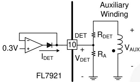
Figure 39. Valley Detection
