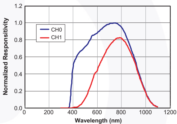
Fig. 4 Spectral Response
