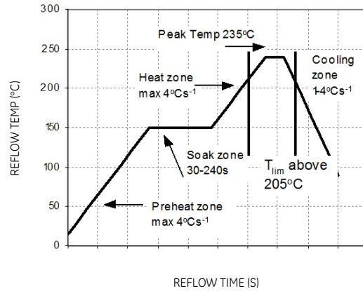
Figure 15: Reflow Profile for Tin/Lead (Sn/Pb) process.
