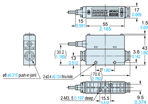
FM-2□-8(-P)
