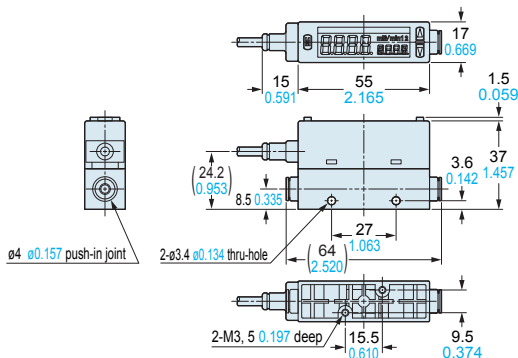
FM-2□-4(-P)
