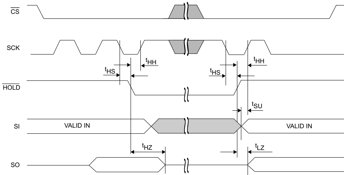
Figure 14. HOLD Timing
