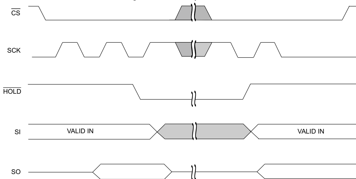
Figure 12. \overline{HOLD} Operation [2]
