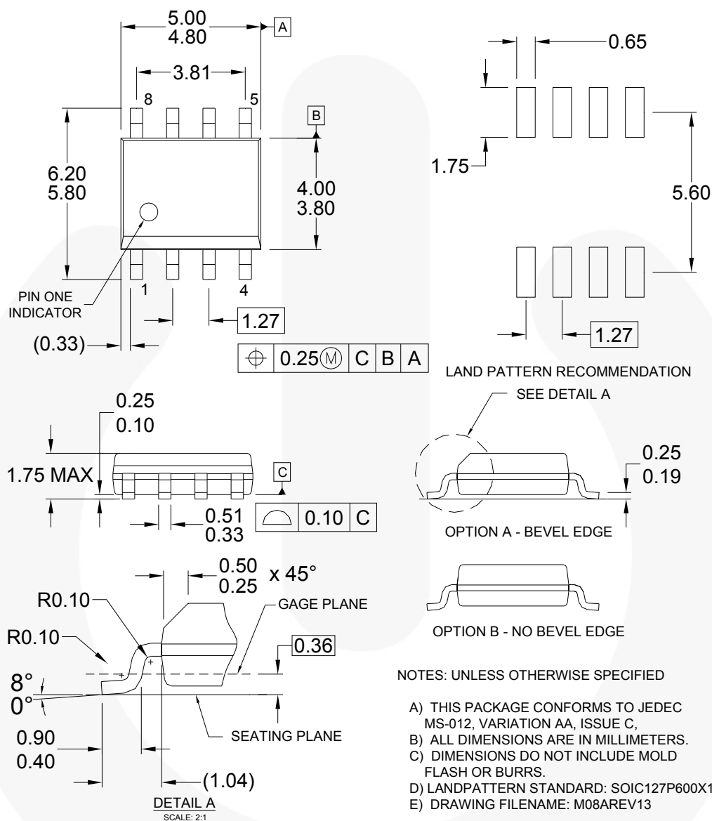
Figure 21. 8-Lead, Small Outline Integrated Circuit (SOIC)
