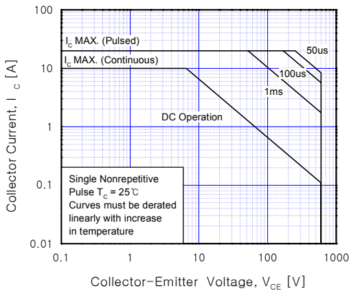
Figure 15. SOA Characteristics
