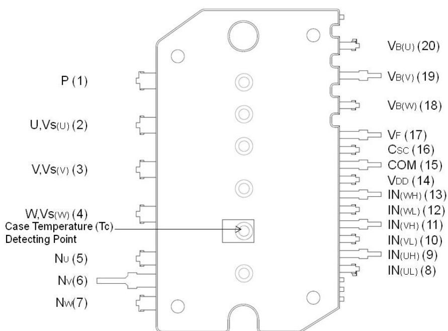
Figure 2. Top View
