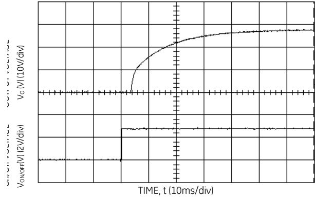
Figure 4. Typical Start-Up Using Remote On/Off, R1=30k\Omega ; C_{o,ext} = 470\mu F .
