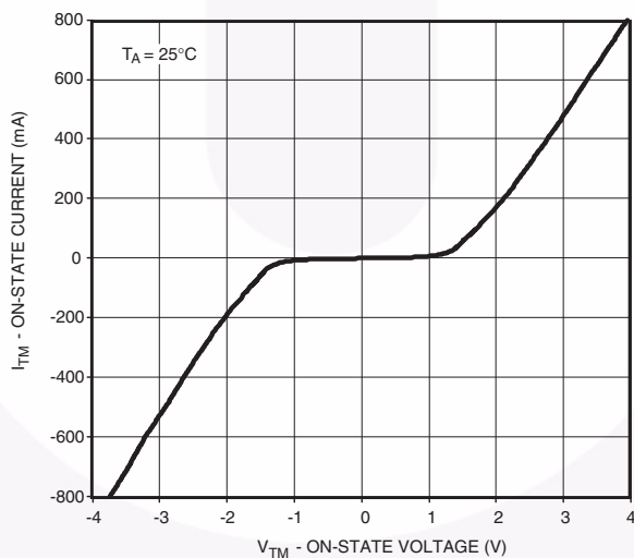
Fig. 9 On-State Characteristics
