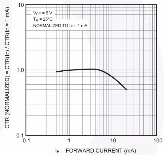
Figure 6. Normalized CTR vs. Forward Current
