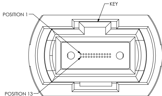
24 FIBER CONNECTOR
