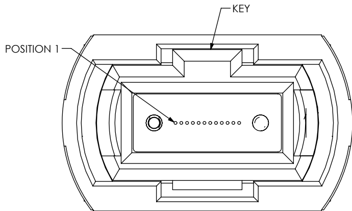
12 FIBER CONNECTOR
