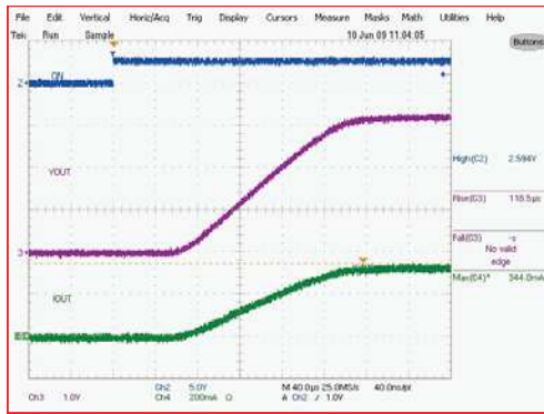
Figure 24. Turn-On Response (V_{IN}=3.3V, C_{IN}=1\mu F, C_{OUT}=0.1\mu F, R_L=100\Omega)
