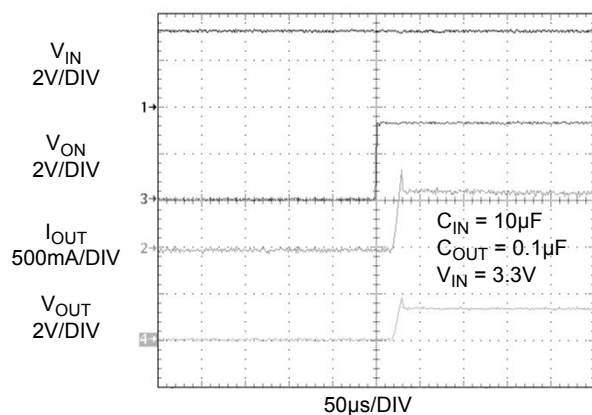
Figure 19. Current Limit Response Time (Output is loaded by 2.2\Omega , C_{OUT} = 0.1\mu F )
