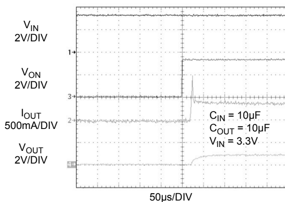
Figure 20. Current Limit Response Time (Output is loaded by 2.2\Omega , C_{OUT} = 10\mu F )
