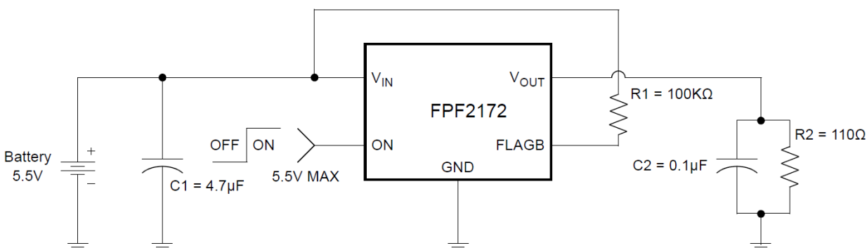
Figure 22. Typical Application
