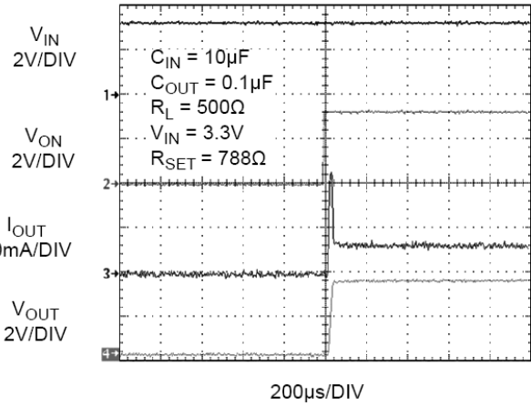
Figure 18. t_{ON} Response
