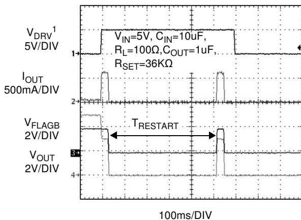
Figure 17. T_{RESTART} Response
