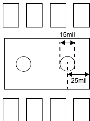
Figure 39. Two Through-Hole Open Vias Embedded in DAP
