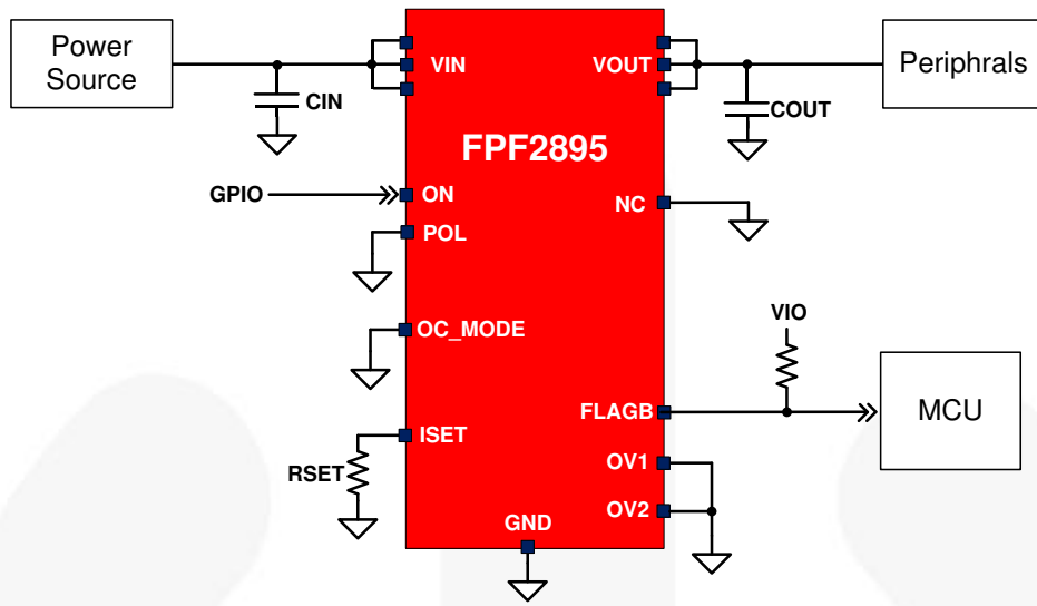
Figure 1. Typical Application
