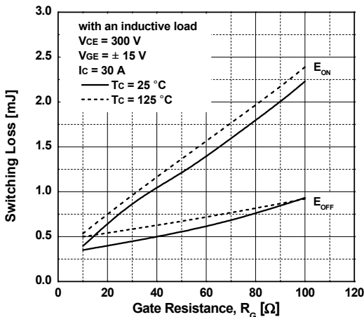
Fig 5. Switching Loss vs. Gate Resistance - Outer IGBT
