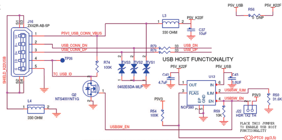
Figure 8. K22F USB port
