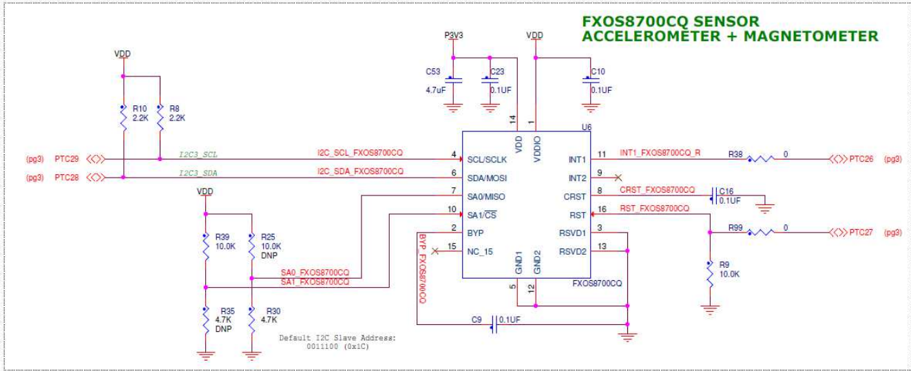
Figure 11. Accelerometer and magnetometer
