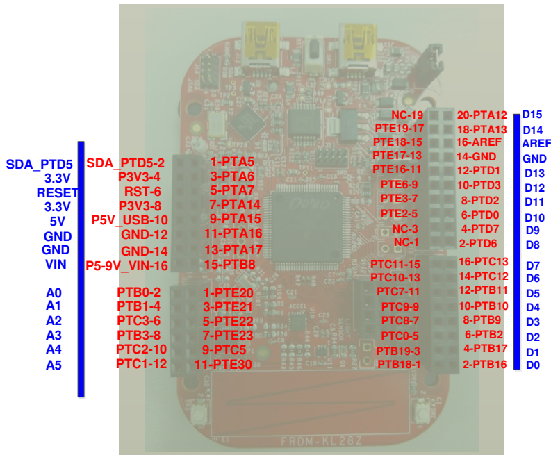
Figure 15. Input/output headers
