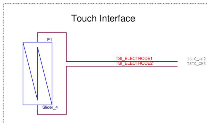
Figure 7. Touch slider connection
