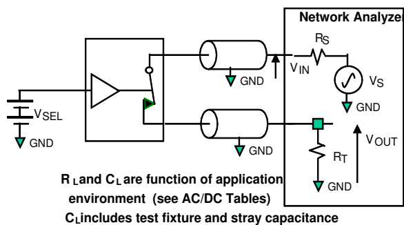
Figure 9. Bandwidth
