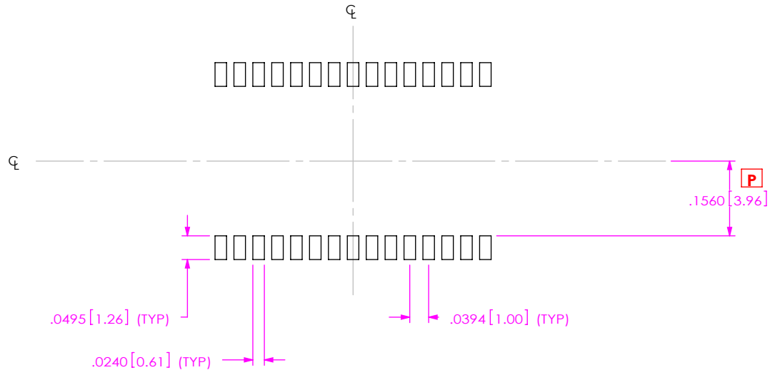
FIG 4 FOR -10, -20, -30 POSITION (THREADED) OR -05 THROUGH -50 (NON-THREADED) ALL DIMENSIONS ARE SYMMETRIC ABOUT THE CENTERLINE.
