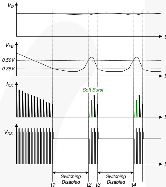
Figure 26. Burst-Mode Operation
