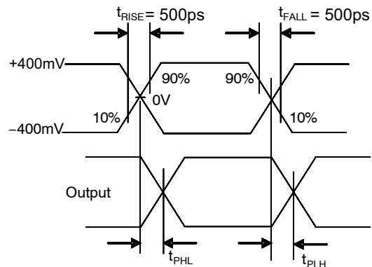
Figure 11. Intra-Pair Skew Test t_{SK(P)}
