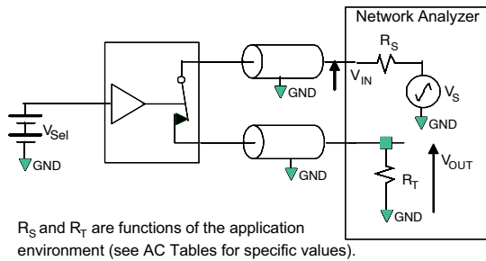
Figure 13. Bandwidth
