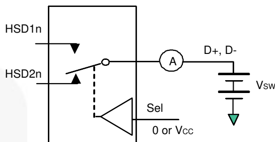
Figure 5. Off/On Leakage
