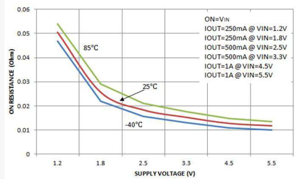
Figure 17. R_{ON} vs. Supply Voltage
