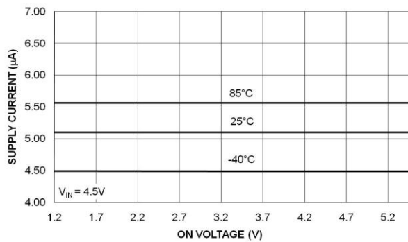
Figure 12. Quiescent Current vs. On Voltage (V BAT =4.5 V)
