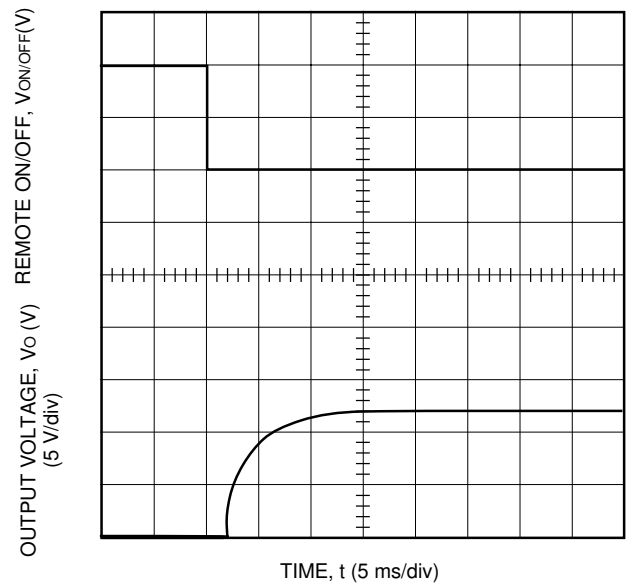
Figure 7. Typical FW300B1 Start-Up Transient at Room Temperature, 48 V Input, and Full Load
