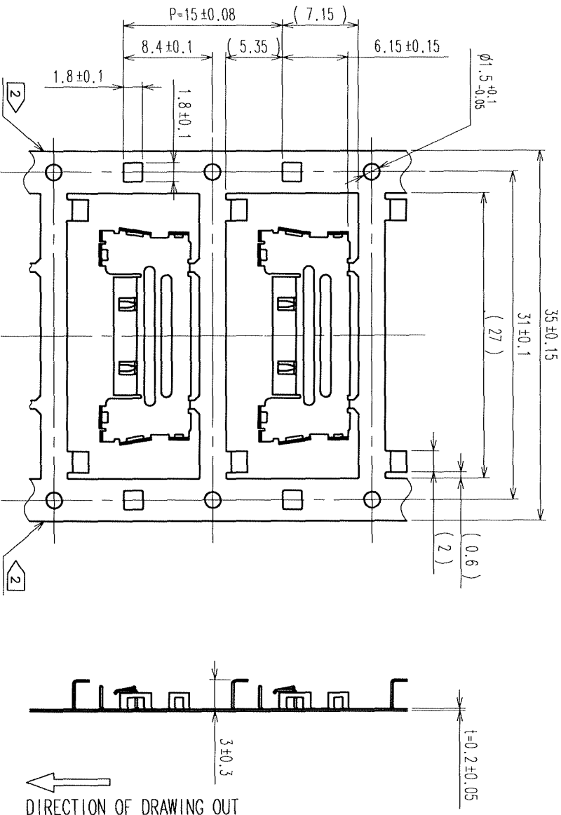
DETAILED FIGURE OF CARRIER ( 2 : 1 )
