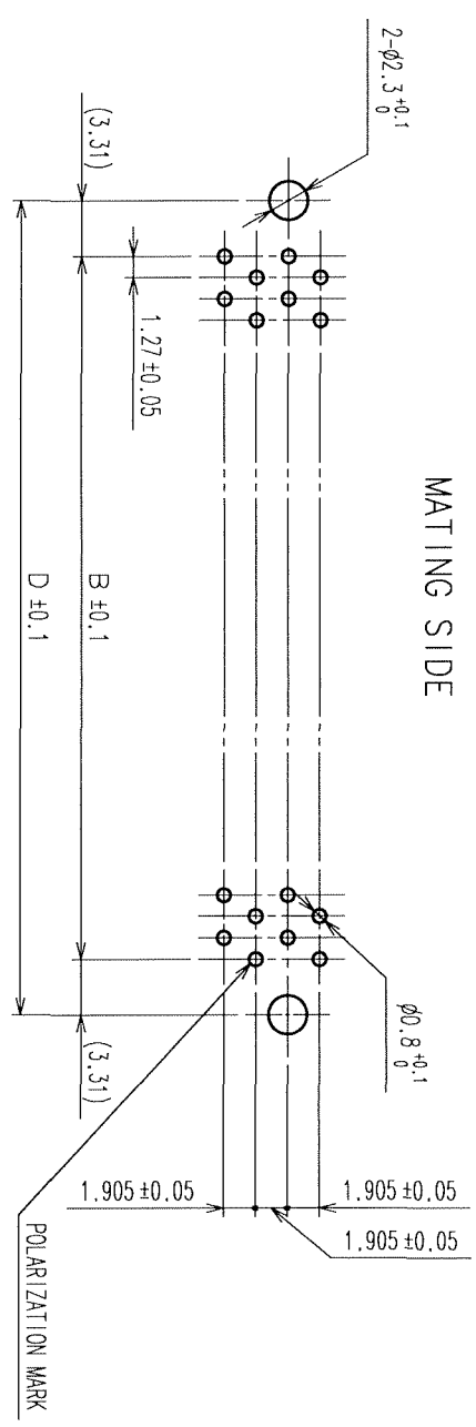
RECOMMENDED PC BOARD HOLE PATTERN (MOUNTING SIDE) t=1.6
