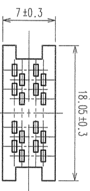
PROTECTOR (A)
