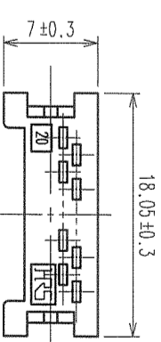
PROTECTOR (B)
