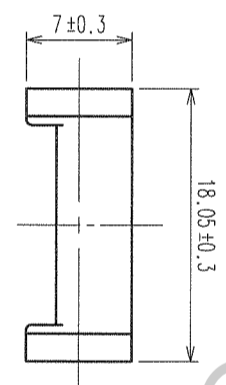
CABLE CLAMP
