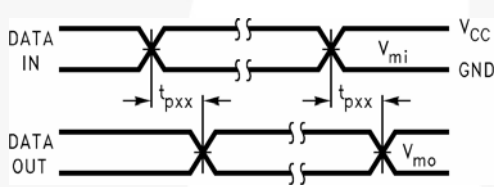
Figure 3. Waveform for Inverting and Non-Inverting Functions
