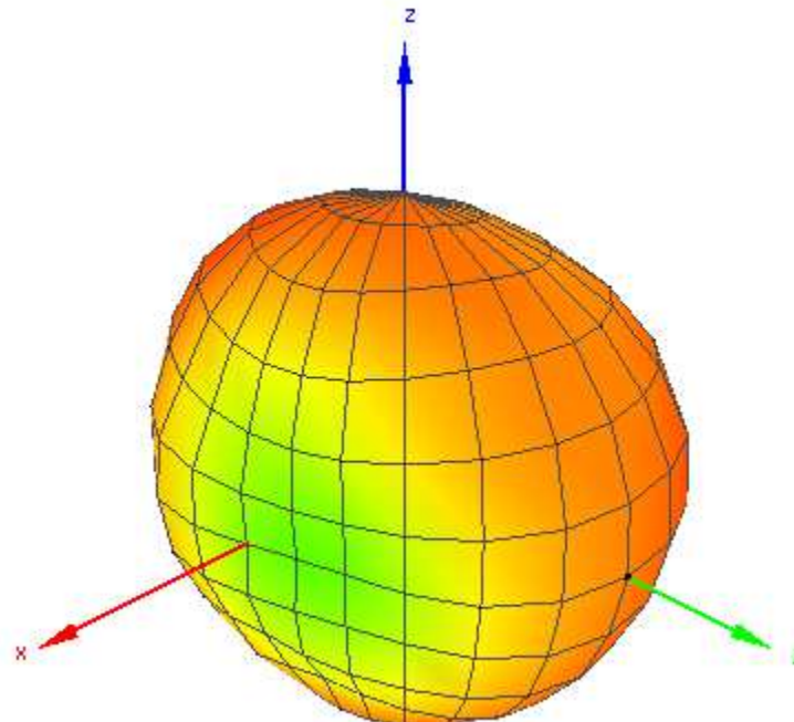
Figure 10. Radiation Pattern at 1400 MHz of FXUB63 Antenna.
