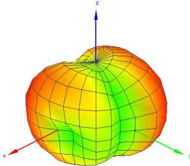
Figure 9. Radiation Pattern at 925 MHz of FXUB63 Antenna.
