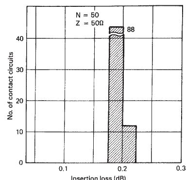
G5Y-1 Distribution of insertion loss at 900 MHz
