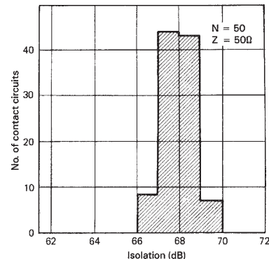
G5Y-1 Distribution of isolation at 900 MHz
