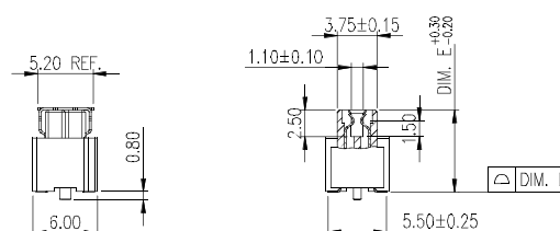
RA-A SECTION
