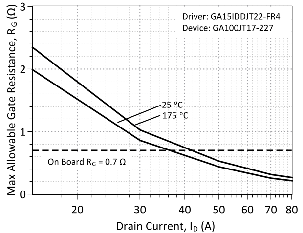
Figure 26: Maximum gate resistance for safe operation of the GA100JT17-227 at different drain currents using the GA15IDDJT22-FR4 board.
