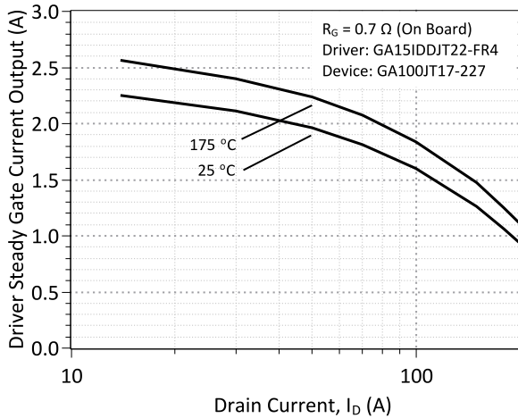
Figure 25: Typical steady state gate current supplied by the GA15IDDJT22-FR4 board for the GA100JT17-227 with the on board resistance of 0.7 Ω
