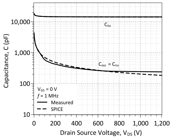
Figure 9: Input, Output, and Reverse Transfer Capacitance
