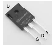
TO-247
