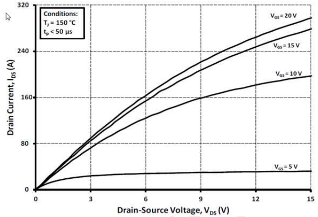
Typical Forward Characteristics T j =25 °C
