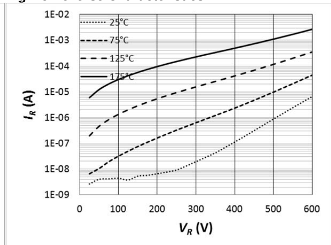
Fig. 18 Reverse Characteristics
