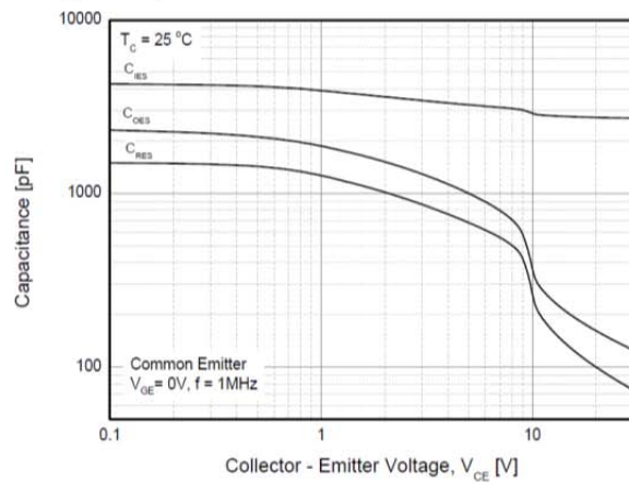
Fig. 6 Capacitance characteristics
