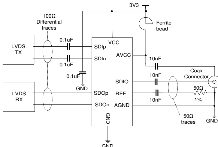
Figure 8: Example Schematic Implementation for EQCO850SC-HS. For EQCO875SC-HS replace the two 50\Omega references with two times 75\Omega .
