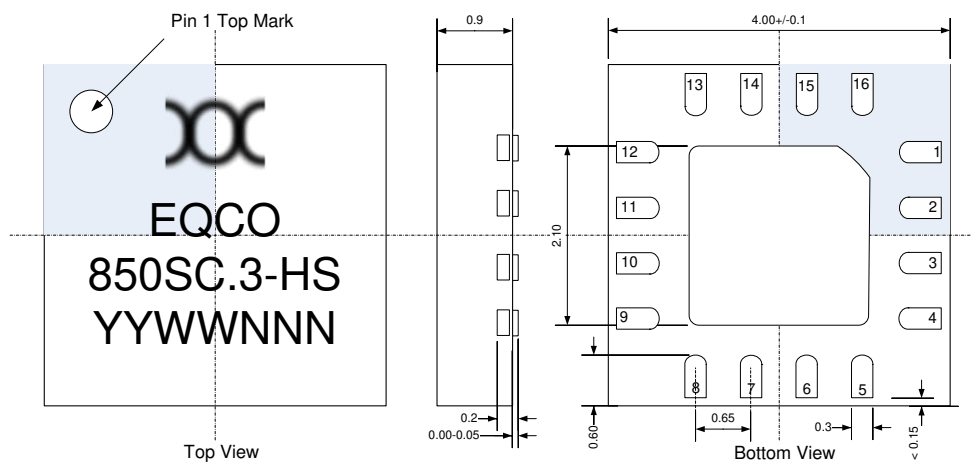
Figure 6: Package Drawings
