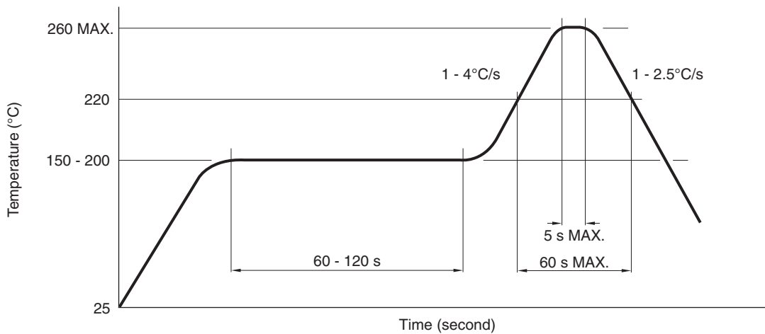
Fig. 17 Temperature Profile
