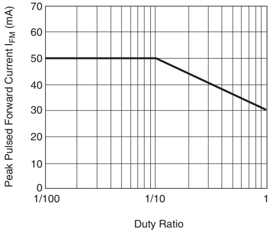
Fig. 2 Peak Pulsed Forward Current vs. Duty Ratio
