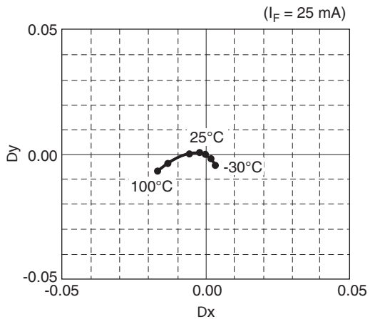
Fig. 9 Relative Chromaticity vs. Case Temperature
