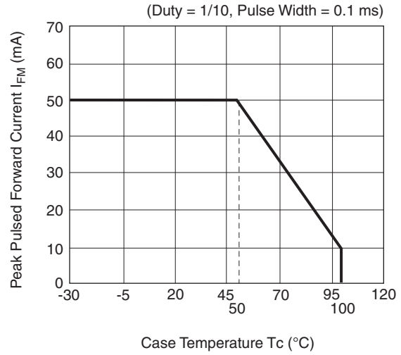
Fig. 3 Peak Pulsed Forward Current vs. Case Temperature
