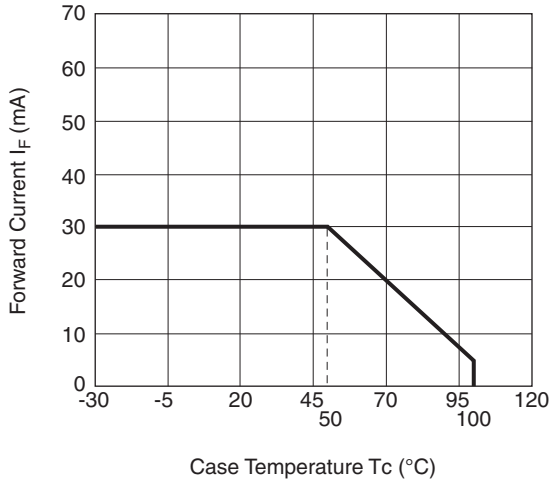
Fig. 1 Forward Current vs. Case Temperature
