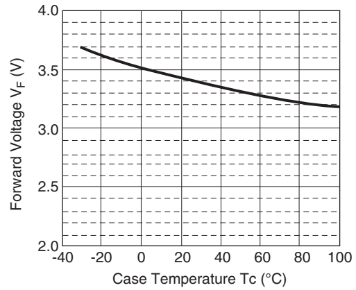
Fig. 7 Forward Voltage vs. Case Temperature
