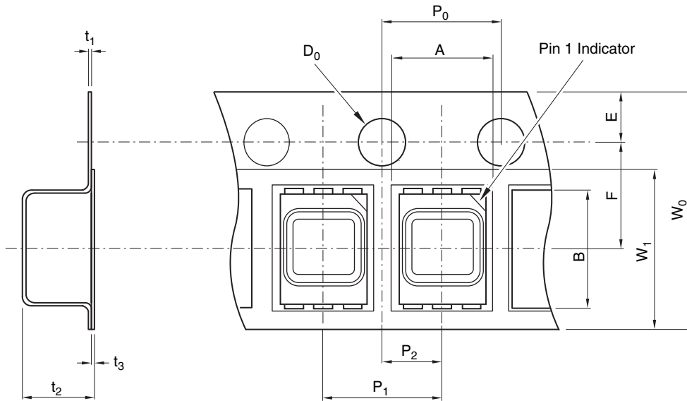
Fig. 11 Tape Shape and Dimensions
