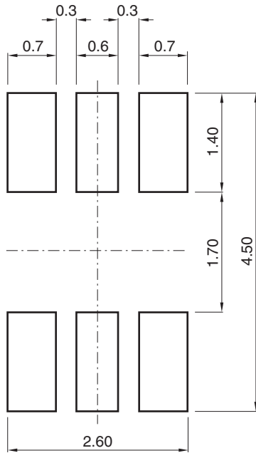
Fig. 18 Recommended Solder Pad Design
