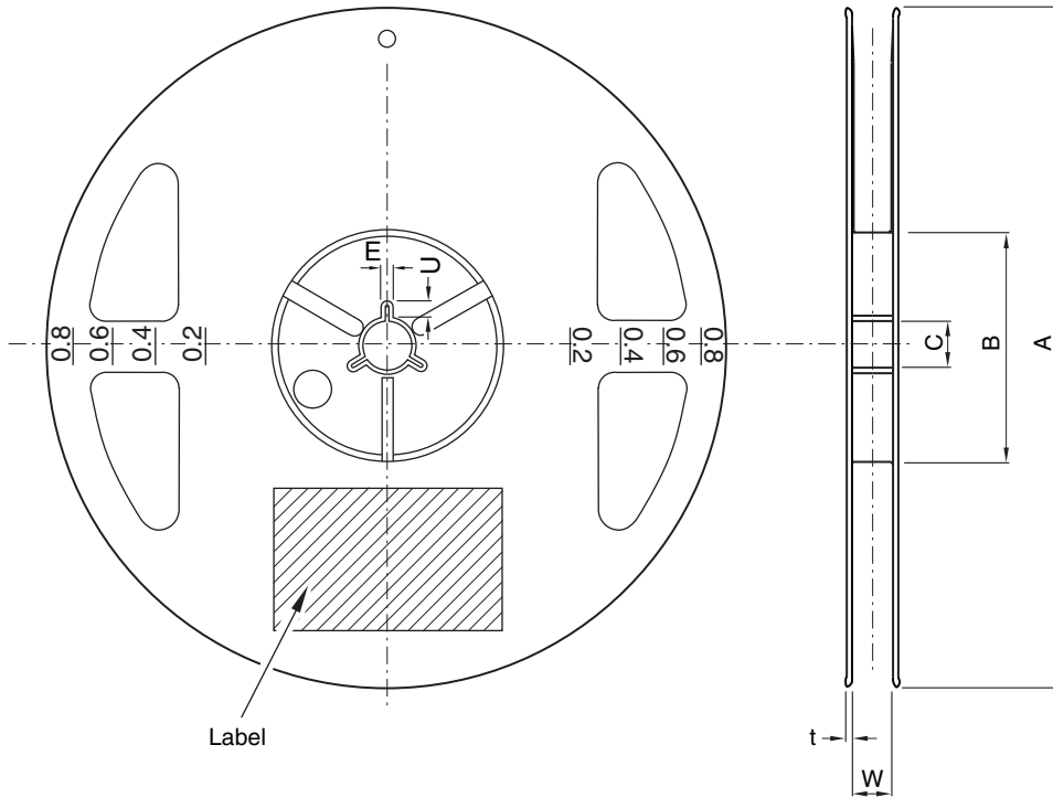
Fig. 12 Reel Shape and Dimensions
