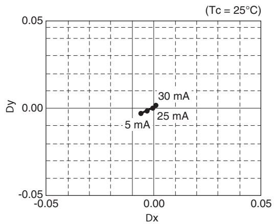
Fig. 8 Relative Chromaticity vs. Forward Current
