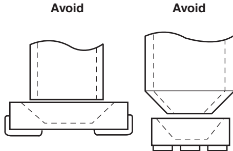
Fig. 19 Recommended Nozzle
