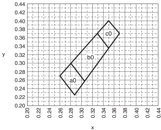
Fig. 10 Chromaticity Diagram
