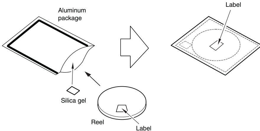
Fig. 16 Factory Moisture-proof Packing
